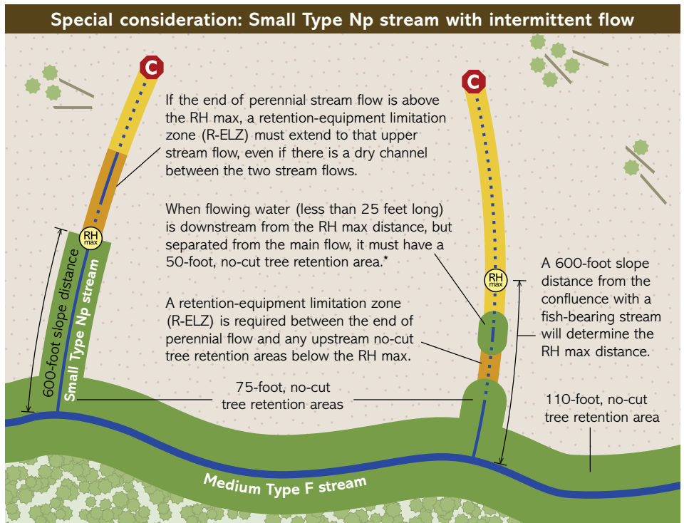
Note: This diagram uses westside, standard practice measurements, but the concepts illustrated apply to both sizes of forestland and in both regions of Oregon.
