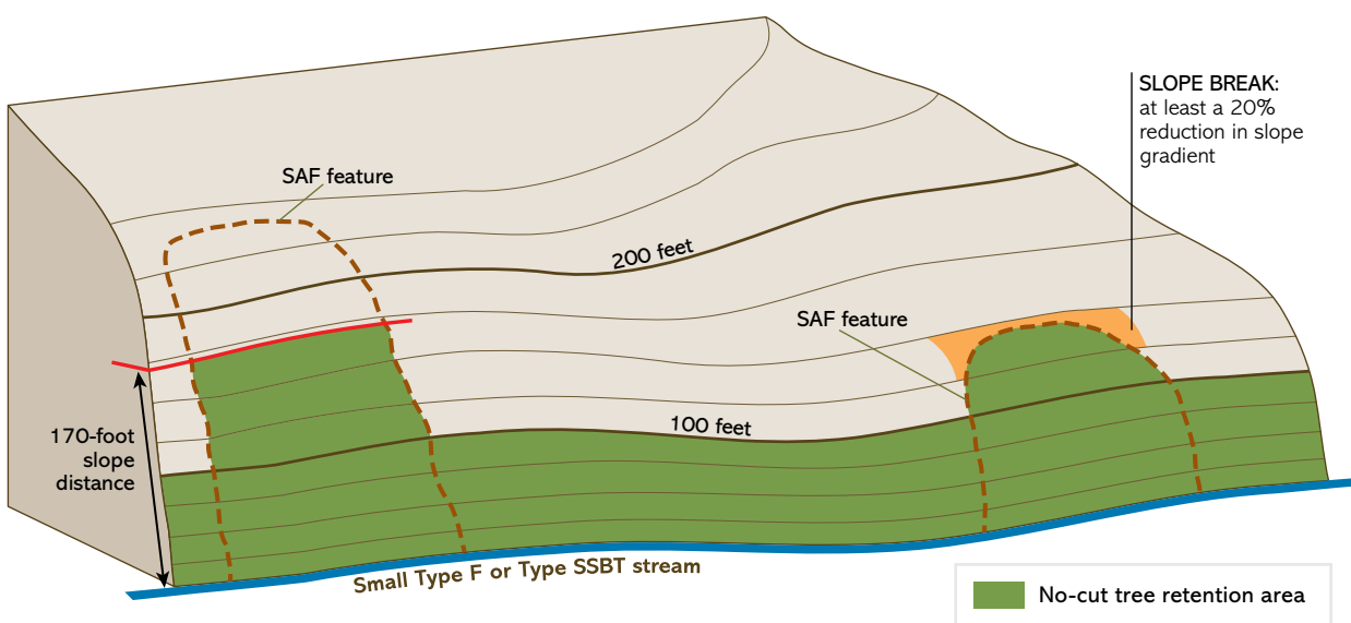
Example of stream-adjacent failures relative to limits imposed on RMA width extension on Type F and Type SSBT streams.
